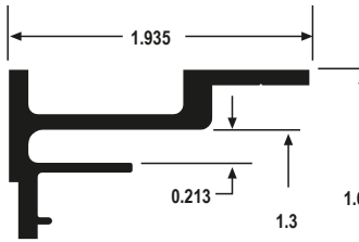
37894s ACM Female Connector 6063-T6 x 12h'
