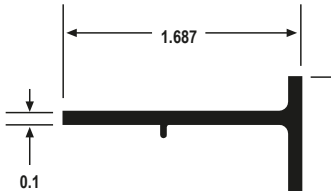
37893s ACM Terminator Connector 6063-T6 x 12' Mill finish
