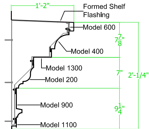
COMPONENTS & GUSSET ASSEMBLY CORNICE DESIGN 10EX - Expanded for Dentils
