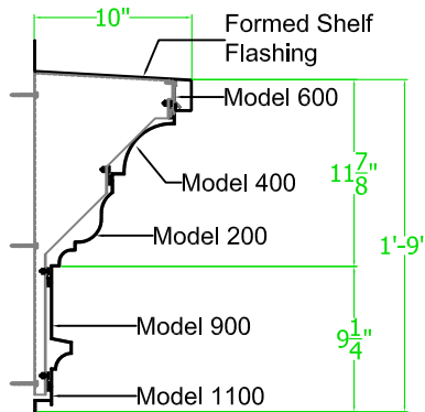
COMPONENTS & GUSSET ASSEMBLY
