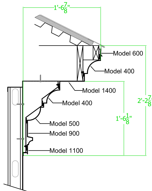
ASSEMBLY AT EAVE GUSSET
