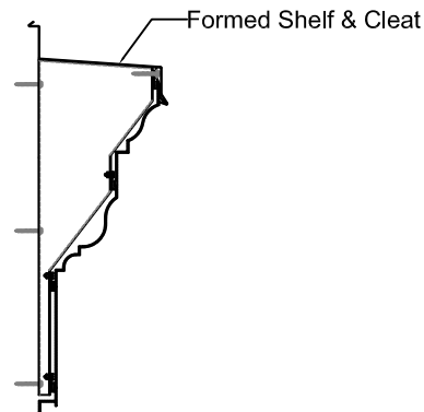
ASSEMBLY AT PARAPET
