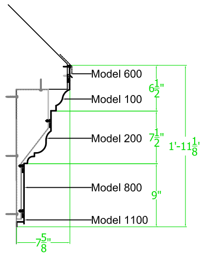
ASSEMBLY AT EAVE
