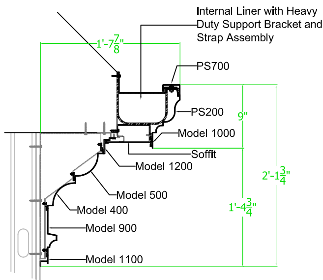
ASSEMBLY AT EAVE
