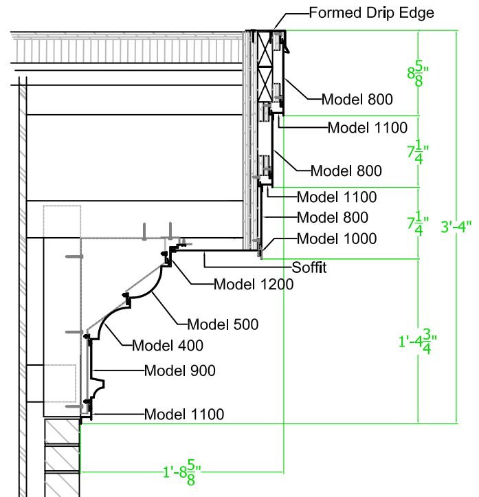
ASSEMBLY AT GABLE
