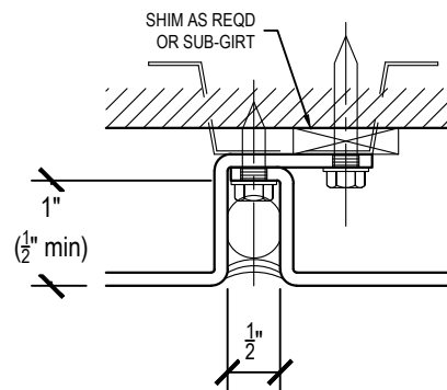
TYPICAL DETAIL
