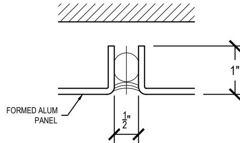
TYPICAL DETAIL
